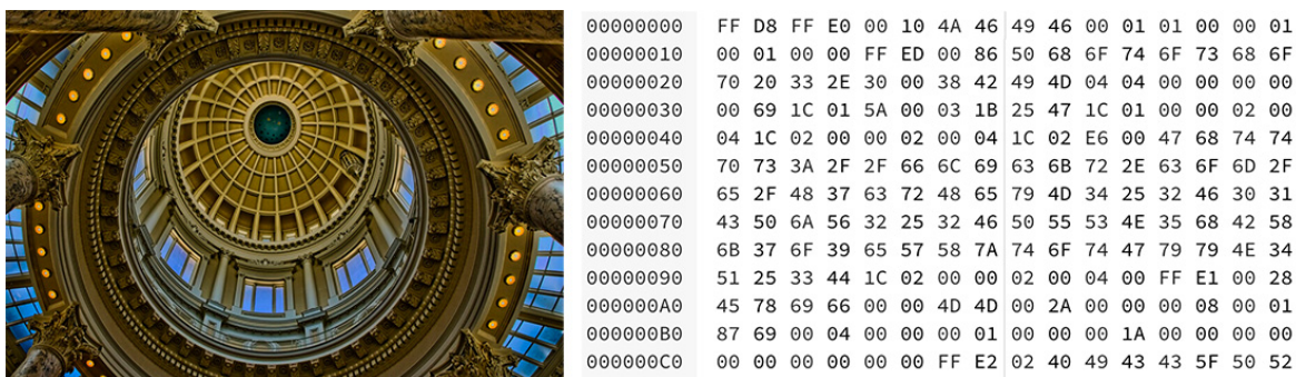
Figure 19. Raw data of a .jpg image file
